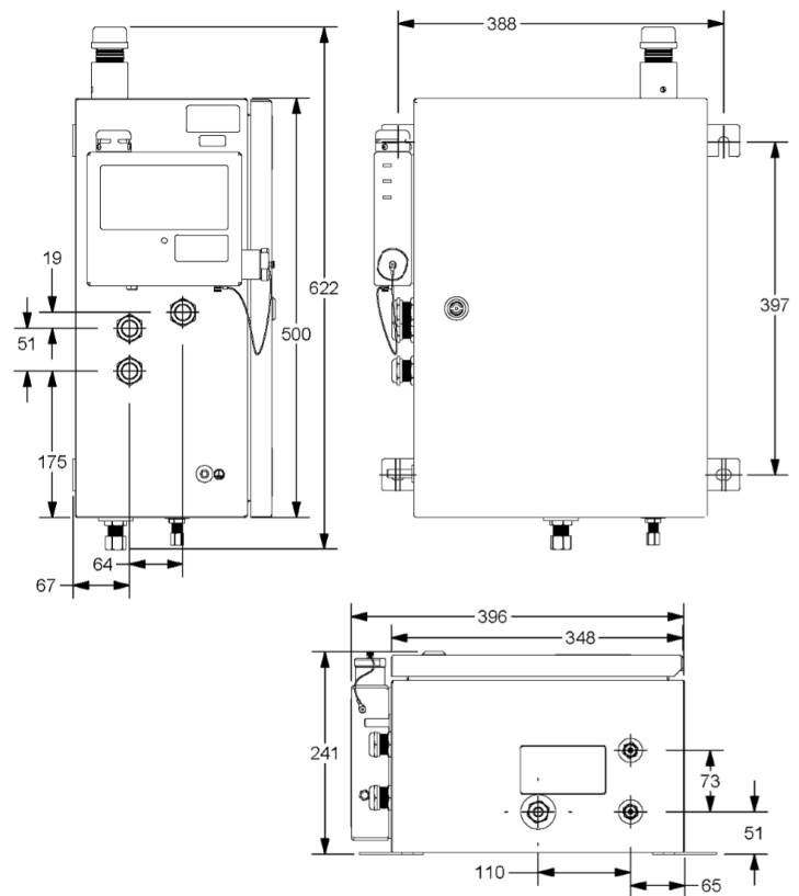
Figure 4: Overall Mounting Dimensions of the Instrument
