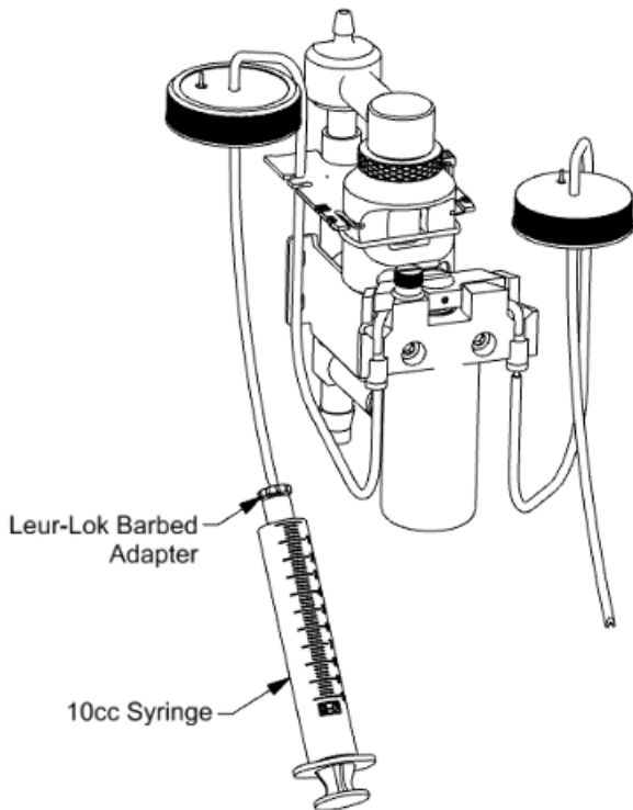
Figure 6: Check Valve Flushing
