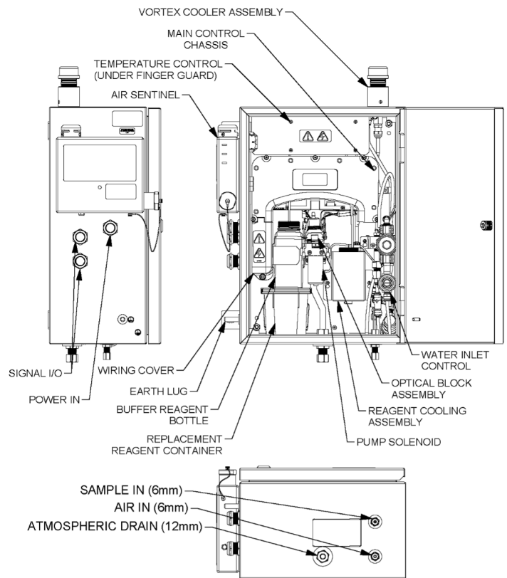
Figure 3: The CLX-Ex with Cover Open
