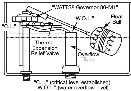
TYPICAL WATER CLOSET
