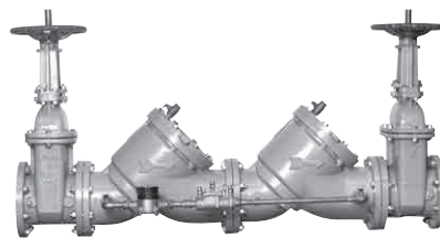
Watts Series 709DCDA
